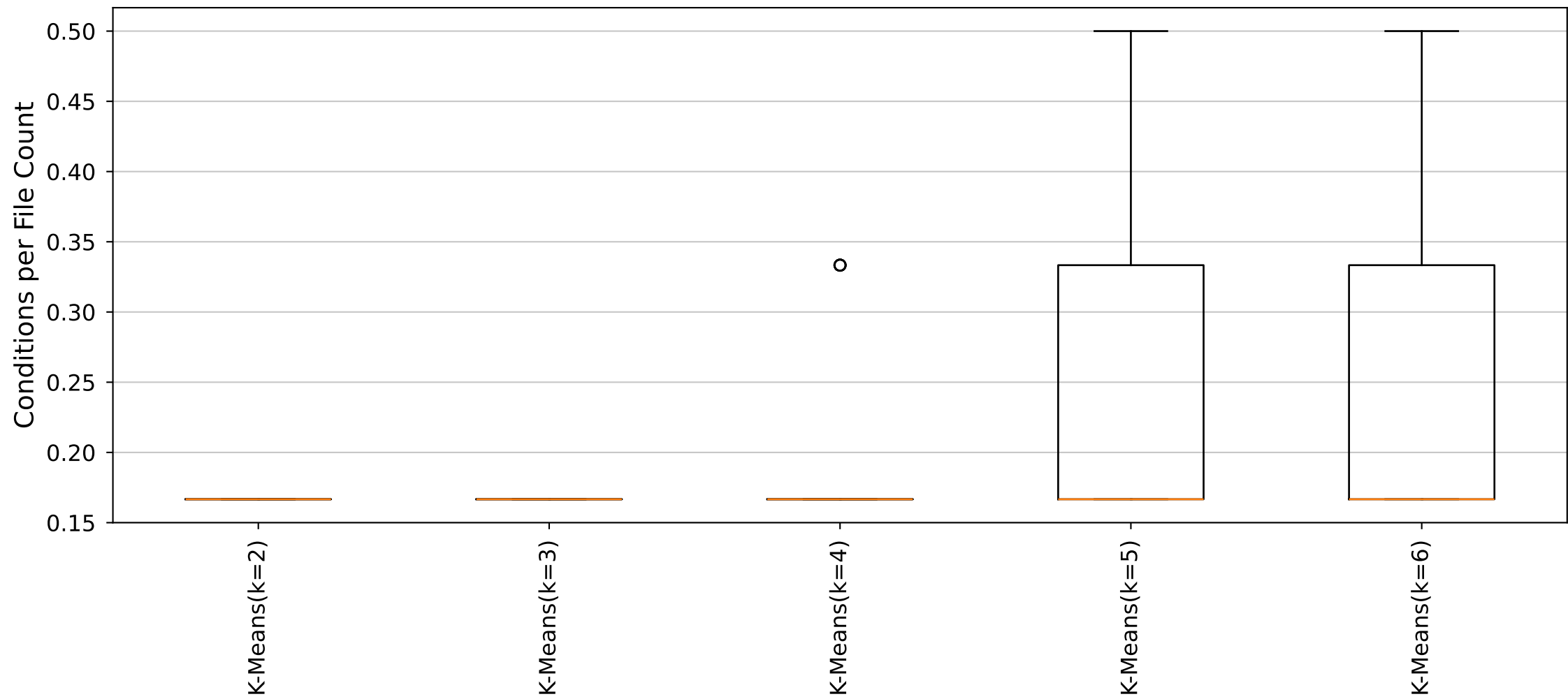
YARA Rules Conditions per File Count Distribution (Cluster22_Size6 dataset)
